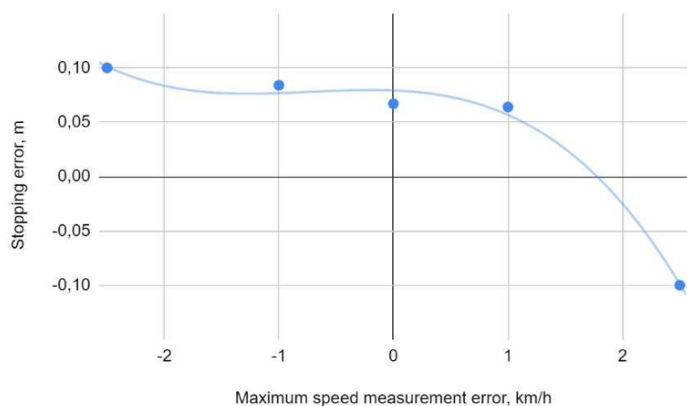
Fig. 8. Impact of the speed measurement error on the precision of automatic target braking
